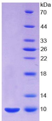
Figure 2. SDS-PAGE
